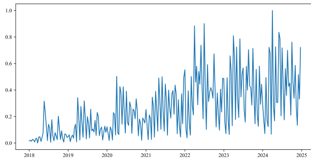
Figure 11: Min-Max scaled
