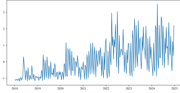
Figure 13: Standard scaled
