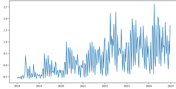
Figure 15: Robust scaled
