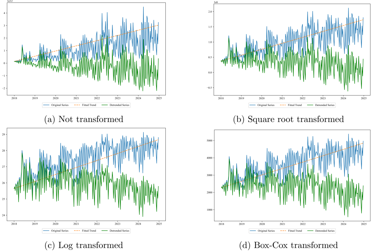
Figure 18: GLS detrending
