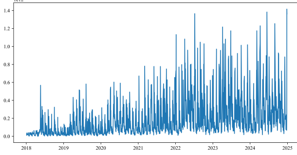
Figure 1: Original series
