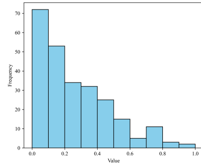
Figure 12: Distribution
