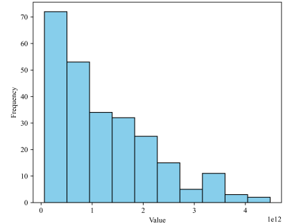
Figure 4: Distribution
